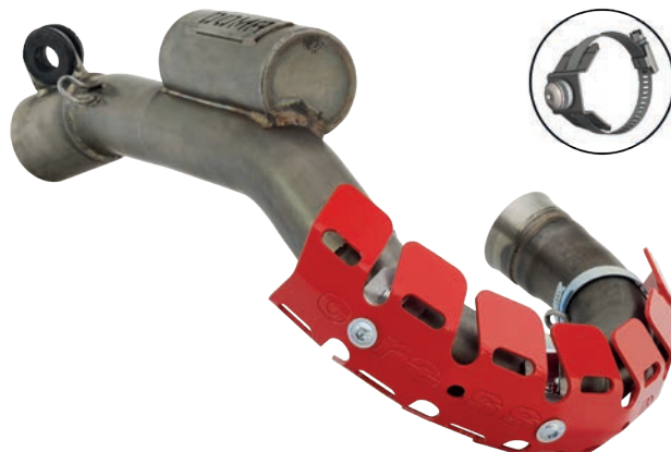
2 STROKE EVO SKU: 2CP0730003_ with clamp "easy fixing"
